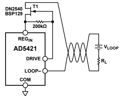
Figure 43. MOSFET Connecting the AD5421 to Loop Power Supply
