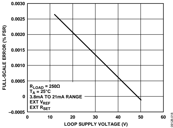
Figure 19. Full-Scale Error vs. Loop Supply Voltage
