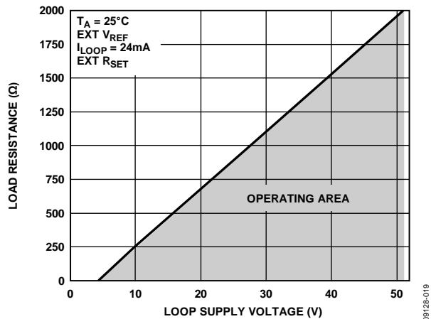
Figure 20. Load Resistance Load Line vs. Loop Supply Voltage (Voltage Between LOOP- and REG_{IN} )
